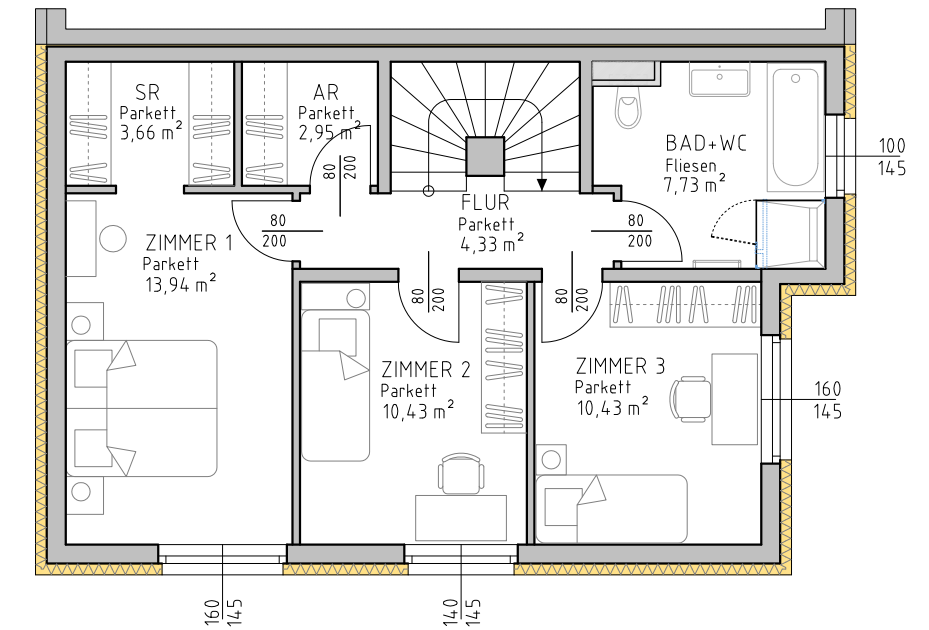
1.STOCK
